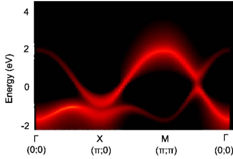
FIG. 2. (Color online) LDA+DMFT+ \Sigma_k quasiparticle energy dispersion of PCCO Cu- 3d(x^2-y^2) orbital for high symmetry directions of square Brillouin zone. The Fermi level is zero. Here and below intensity goes down as yellow-red-black.
