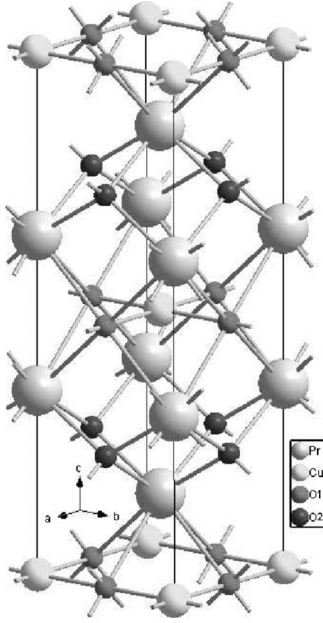
FIG. 1. The crystal structure of \text{Pr}_2\text{CuO}_4 . Medium size gray spheres correspond to the copper atoms, small dark and black spheres are O1 and O2 atoms, respectively, and big gray spheres correspond to praseodymium atoms.
