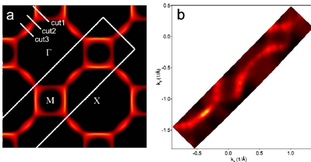
FIG. 3. (Color online) (a) Extended Fermi surfaces for PCCO-LDA+DMFT+ \Sigma_k data. White rectangle in (a) schematically shows the part of reciprocal space measured experimentally (b). Lower left corner is X point ( \pi, 0 ).
